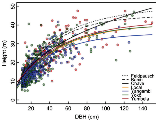
Fig. 2 Height-diameter models for the studied region, namely, the local model (orange) and the mixed effects local model with site-specific deviations for Yangambi (blue), Yoko (green), and Yambela (red). The regional models for central Africa by Feldpausch et al. (2012) (black dotted line) and Banin et al. (2012) (black dashed line) and the pan-tropical model by Chave et al. (2014) (full black line) are indicated
